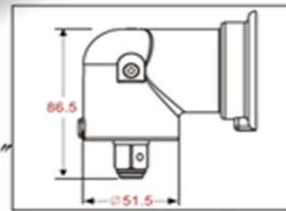
OP-130LH4 1/2" Side exhaust 側排氣
